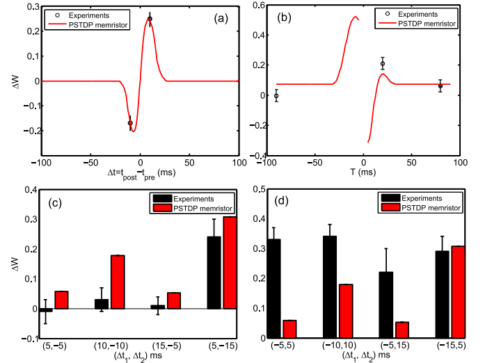
Fig. 6. (a) Pair-based STDP memristive synapse of [19] reproduces the STDP learning window, while it fails to generate (b) quadruplet data, and cannot distinguish between (c) pre-post-pre, and (d) post-pre-post triplet.
