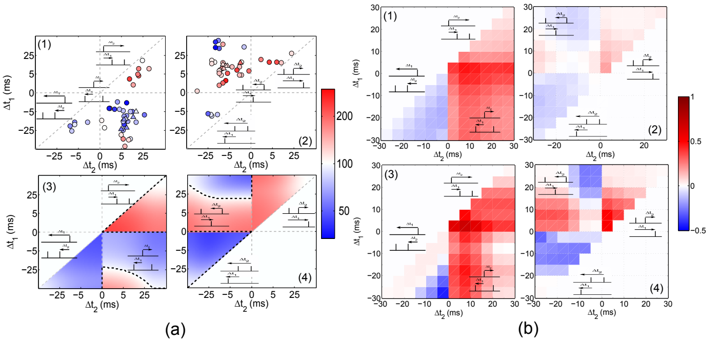
Fig. 8. (a1-a2) Experimental triplet data of [8] for six different spike triplet combinations. (a3-a4) A suppressive PSTDP model proposed by Froemke and Dan approximate the experimental data. (b1-b4) The proposed triplet-based STDP memristive synapse mimics the weight modifications data and suppressive PSTDP model of [8]. (b1-b2) show weight changes produced using the optimized parameters for the triplet case of hippocampus experiments under scenario 1, i.e. when NMSE = 3.61 (see Table I). (b3-b4) similar to (b1-b2), except that the parameters used for generating the weight changes are those utilized to reach an NMSE of 0.87, i.e. the triplet case of hippocampus experiments under scenario 2 (see Table I). The contrast between weight changes in the post-pre-post case is due to the difference between the suppressive PSTDP model of [8] and the TSTD model of [14] that is implemented in this paper. In (a), the colorbar shows normalized weight changes obtained from the experiments. However, the colorbar in (b) demonstrates the exact values for weight changes obtained using the proposed circuit.
