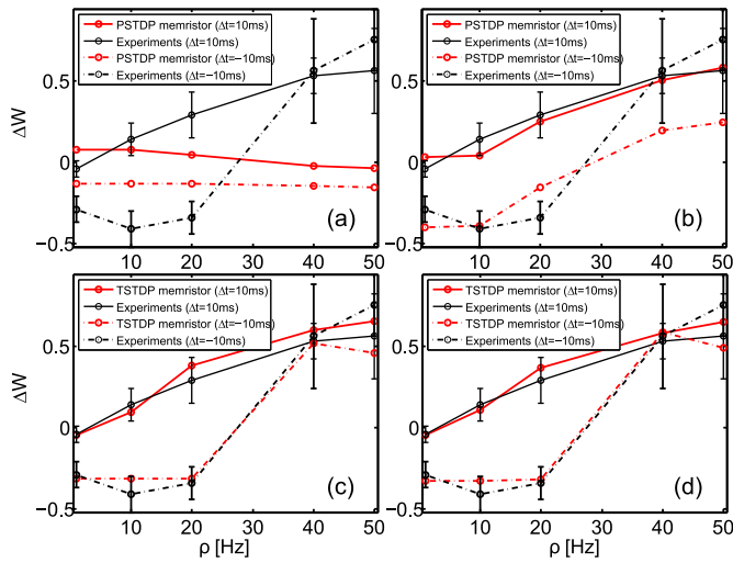
Fig. 5. (a) Pair-based STDP memristive synapse of [19] fails to mimic experimental data of [12], under scenario 1. (b) Similar to (a), only for scenario 2. (c-d) The proposed triplet-based STDP memristive synapse successfully mimics experimental data, under scenario 1 shown in (c) and scenario 2 presented in (d). Here \rho represents the frequency of spike pairs with time differences of 10 ms and -10 ms.
