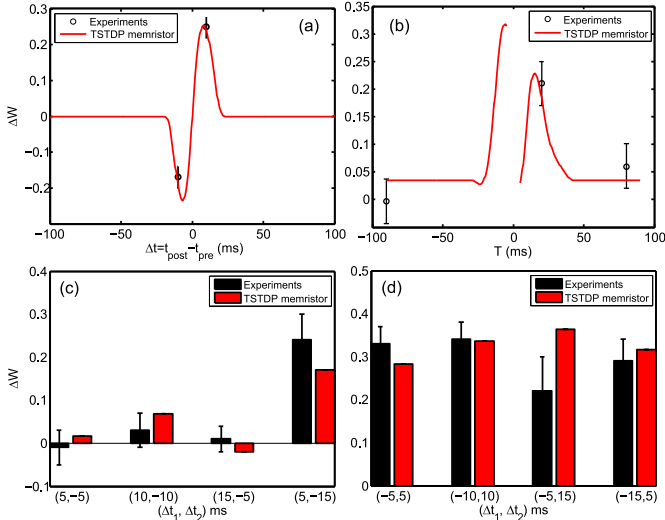
Fig. 7. (a) Proposed triplet-based STDP memristive synapse reproduces the STDP learning window. (b) The proposed TSTDP device predicts similar weight changes to the data presented in [14] for quadruplet protocol. Note that there is no experimental data available around 0 ms. (c)-(d) The proposed synapse, correctly distinguishes between (c) pre-post-pre triplet case, and (d) post-pre-post triplet case.
